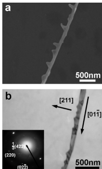
Figure 9. SEM (a) and TEM (b) images of toothed gold nanobelts obtained after reacting at 4 °C for 30 min and then 10 min at 27 °C. (Inset) ED pattern corresponding to the whole region of b.
