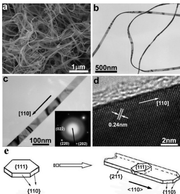
Figure 1. SEM (a), TEM (b,c), and HRTEM (d) images of gold nanobelts obtained at 4 °C. (e) Schematic illustration of the growth direction of gold nanobelts. (Inset) ED pattern corresponding to the whole region of c.
