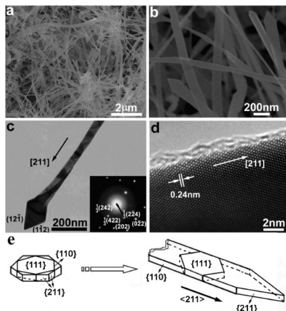
Figure 3. SEM (a,b), TEM (c), and HRTEM (d) images of gold nanobelts obtained at 27 °C. (e) Schematic illustration of the growth direction of the gold nanobelts. (Inset) ED pattern corresponding to the whole region of c.
