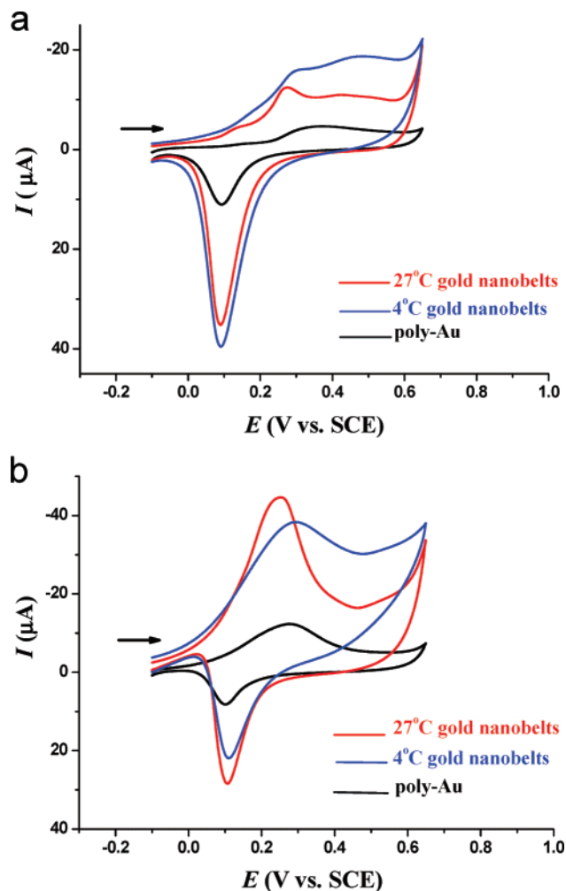
Figure 10. Cyclic voltammograms of gold nanobelt electrodes and polycrystalline Au (poly-Au) electrode in 0.1 \text{mol dm}^{-3} KOH solutions in the absence (a) and presence (b) of 1.0 \text{mol dm}^{-3} \text{CH}_3\text{OH} . The potential scan rate was 10 \text{mV s}^{-1} .
