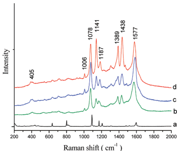
Figure 11. Raman spectrum of solid PATP (a), and SERS spectra of PATP molecules adsorbed on different substrates: (b) \sim 50 nm gold nanoparticles; (c) gold nanobelts obtained at 27 °C; (d) gold nanobelts obtained at 4 °C.
