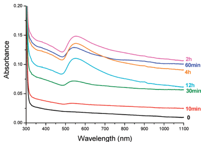
Figure 4. UV-vis absorption spectra of the gold products obtained at 27 °C at different reaction times.
