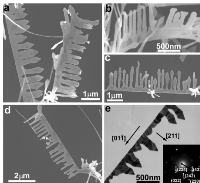
Figure 6. SEM (a–d) and TEM (e) images of gold nanocombs obtained by a two-step process with temperature changing from 4 to 27 °C. (Inset) ED pattern corresponding to the whole region of e.
