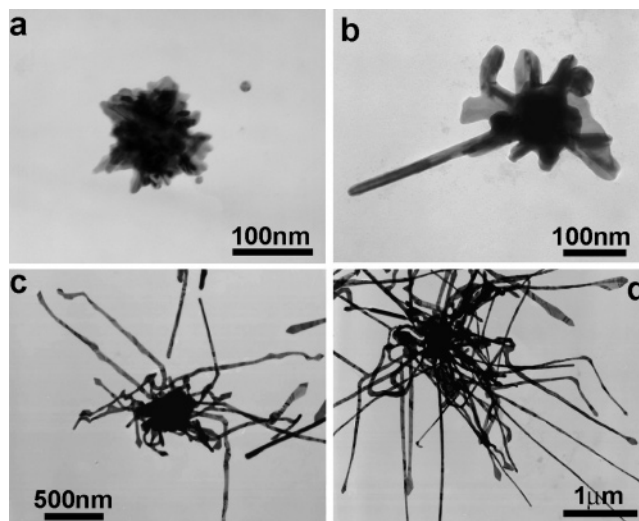
Figure 5. TEM images of gold products obtained at early stages of the gold nanobelts formed at 27 °C: (a) 15, (b) 30, and (c,d) 60 min.
