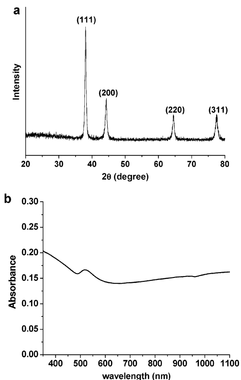
Figure 2. XRD pattern (a) and UV-vis absorption spectrum (b) of gold nanobelts obtained at 4 °C.
