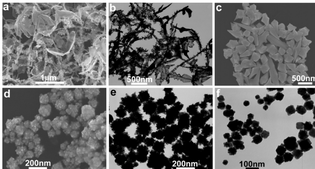
Figure 7. SEM (a,c,d) and TEM (b,e,f) images of gold nanostructures obtained at 4 (a,b,d,e) and 27 °C (c,f) in aqueous solutions of single surfactant: (a–c) 6.5 mM CTAB and (d–f) 1.0 mM SDSn.
