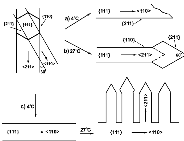
Figure 8. Schematic illustration of the formation mechanism of gold nanobelts and nanocombs. In the upper left corner is presented a projection perpendicular to the top surface of the {111} plane including a hexagonal prism to show the relative angles between different growth directions and side faces of the two kinds of nanobelts.
