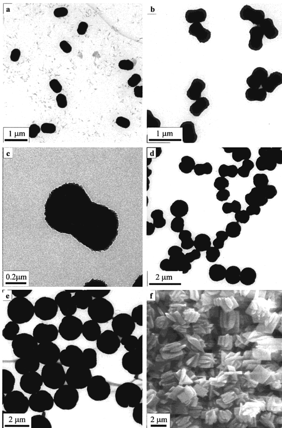
Figure 3. TEM (a–e) and SEM (f) micrographs of \text{BaSO}_4 particles obtained in the presence of PEG- b -PMAA at pH 11 (a), 9 (b, c), 7 (d), 5 (e), and 3 (f).
